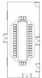
BOARDROOM (CAPACITY 30)
