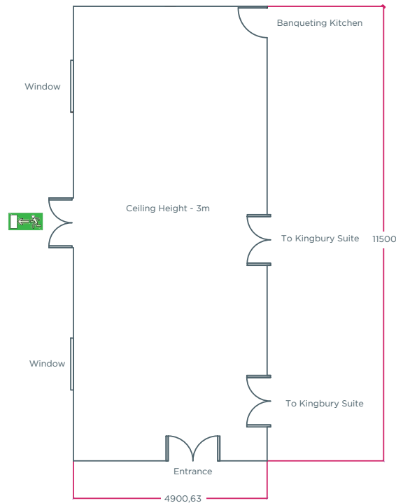
THEATRE (CAPACITY 60)
